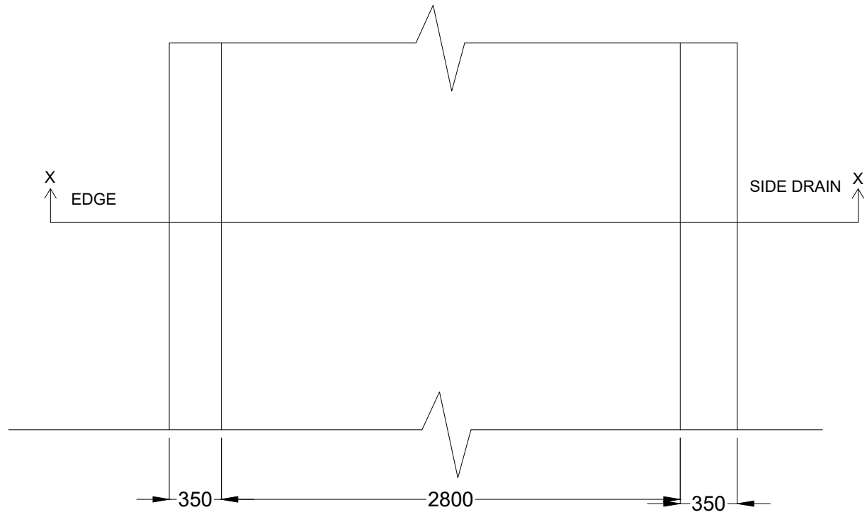
LINK ROAD PLAN
