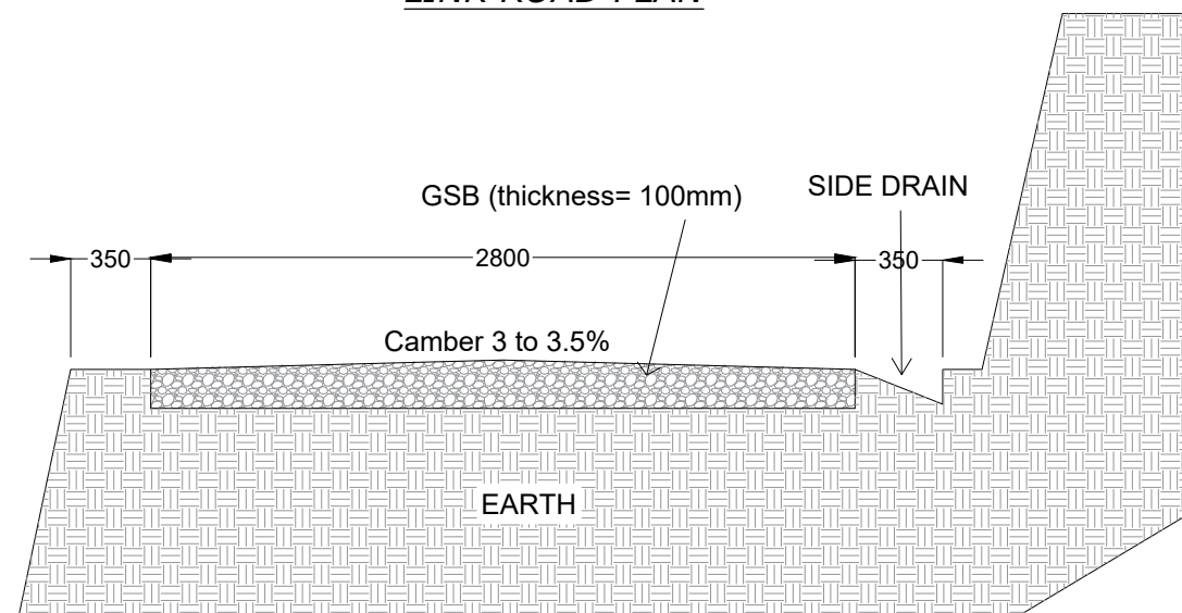
LINK ROAD PLAN
